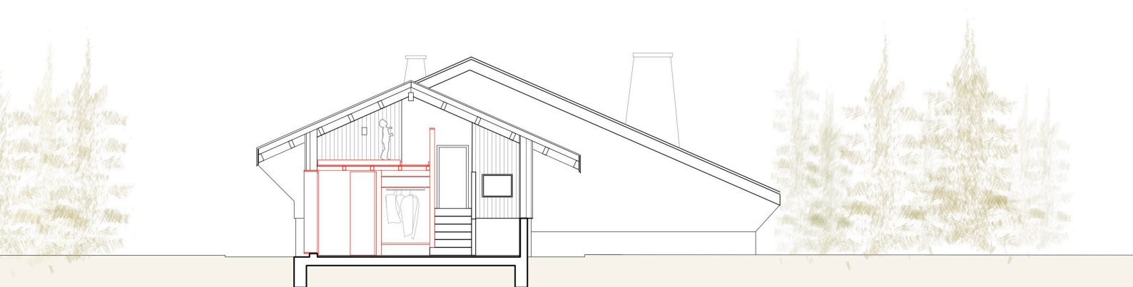
coupe mezzanine
